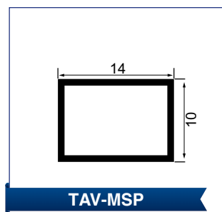
Middle Stick on Profile
