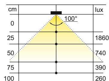
Light Emission Angle
