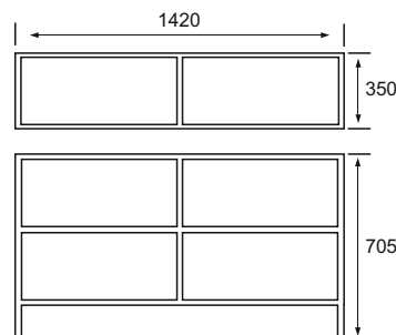
Island Base Rack Material:- Aluminum Alloy Finish:- Black Matte, Brush Gold Size:- 1420x705x350mm
