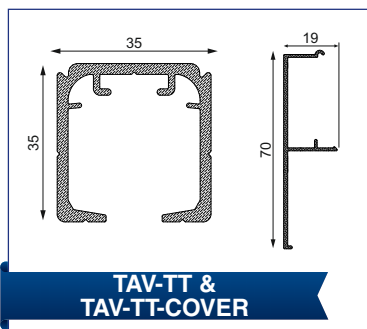
Top Track & Top Track Cover
