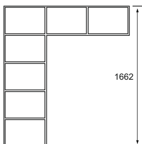
L-Shaped on-wall Combined Rack Material:- Aluminum Alloy Finish:- Black Matte, Brush Gold Size:- 1662x1468x355mm
