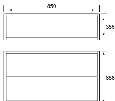
Two layer Aluminum Combined Rack Material:- Aluminum Alloy Finish:- Black Matte, Brush Gold Size:- 850x355x688mm
