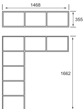
L-Shaped on-wall Combined Rack Material:- Aluminum Alloy Finish:- Black Matte, Brush Gold Size:- 1662x1468x355mm
