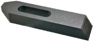
Flat Strap Clamp
