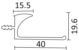
CAP 23 40 MM ALUMINIUM HANDLE PROFILE (3 MTR)
