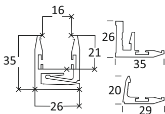
CAP 22 ALLUMINIUM INTERLOCKING GLAZING PROFILE FOR 10/12 MM GLASS
