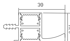
CAP 139 30 MM ALUMINIUM WALL CARCASE GOLA PROFILE WITH LIGHT PROVISION (3 MTR)
