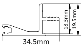
CAP 138 27 MM ALUMINIUM WALL CARCASE GOLA PROFILE (3 MTR)
