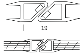
CGS 12 GLASS TO GLASS 180° MAGNETIC 2.2 MTR - 8/10/12MM FIN.: TRANSPARENT
