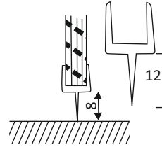
CGS 10 GLASS TO FLOOR PVC 2.2 MTR - 8/10/12MM FIN.: TRANSPARENT
