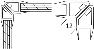
CGS 13 GLASS TO GLASS 90° MAGNETIC 2.2 MTR - 8/10/12MM FIN.: TRANSPARENT
